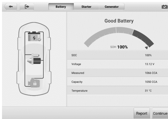
Figure 9-4 Battery Test Results Screen
