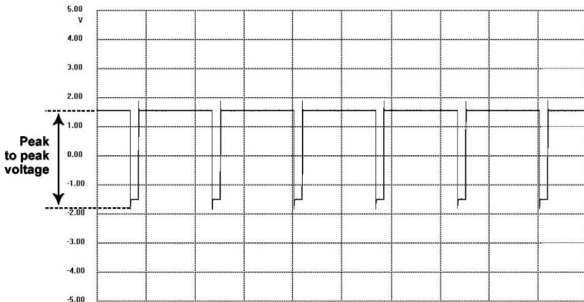
Figure 17-2 Square Waveform
