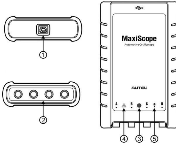
Figure 17-3 MaxiScope Front, Rear, and Top View
