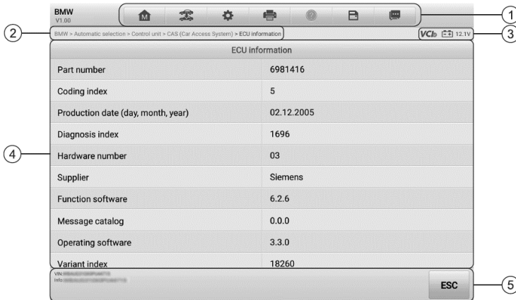
Figure 4-10 ECU Information Screen
