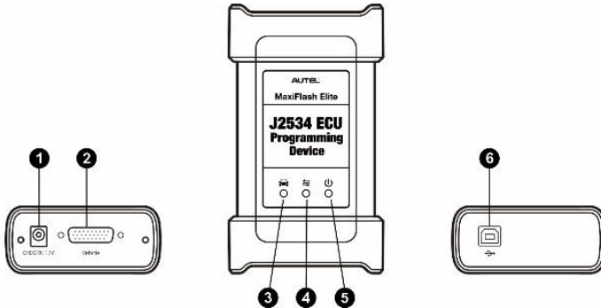
Figure 2-4 J2534 ECU Programming Device
