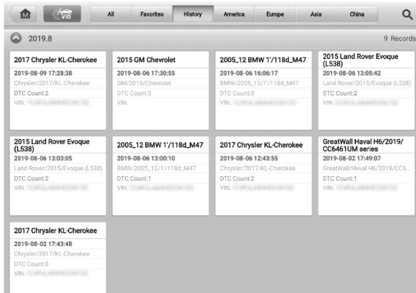
Figure 4-20 History Screen
