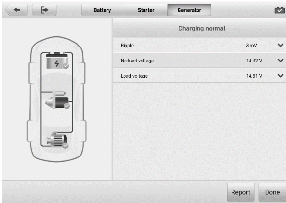
Figure 9-6 Generator Test Results Screen
