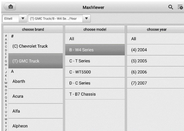
Figure 13-1 MaxiViewer Screen
