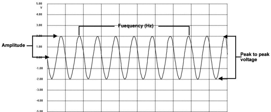
Figure 17-1 Sinusoidal Waveform
