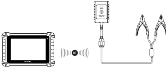
Figure 12-3 Battery Tester Connection Example 1
