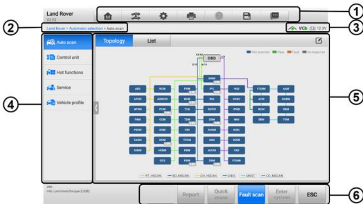
Figure 4-6 Diagnostics Screen
