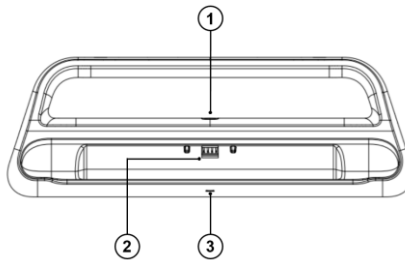
Figure 2-4 Docking Station
